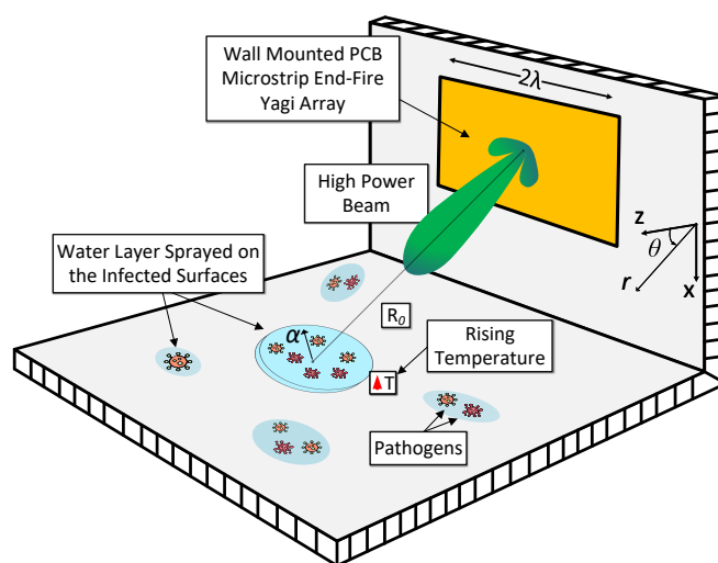
Figure 1. Illustration of the proposed microwave system for thermal sterilization. The transmitting antenna, considered here as a four-element array, could be mounted on a hospital room wall and radiates onto the infected surfaces which are sprayed with a thin water layer.
