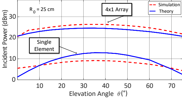
Figure 3. Incident power onto the target in terms of the elevation angle at a distance of 25 cm. The top curves refer to the 4 \times 1 microstrip Yagi array while the bottom are for the planar Yagi single-element antenna (see Fig. 2).
