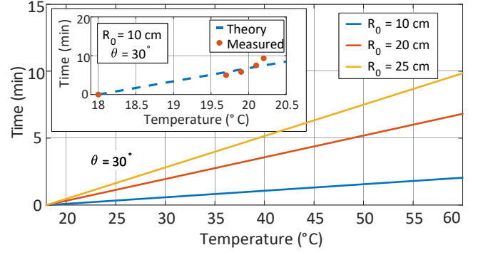
Figure 5. Time versus temperature calculations based on (1) for three different distances whilst considering a 2 W transmitter power. Encapsulated figure: lab measurements as compared to theory for a fixed 10 cm distance, 30^\circ incident angle (see Fig. 4), and a 21.5 dBm transmitter power.
