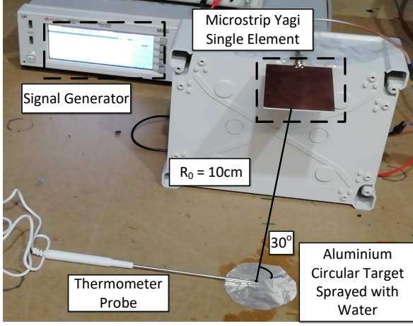
Figure 4. Experimental setup. The target was placed at a 10 cm distance and with an incident angle of 30^\circ with respect to the single-element Yagi antenna.
