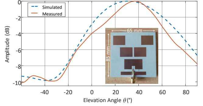
Figure 2. Simulated and measured beam pattern for the single-element planar Yagi designed using microstrip technology. The inset shows the fabricated PCB antenna based on a ROGERS substrate.
